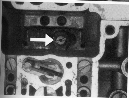
Weber accelerator pump intake valve (arrowed) fitted.
