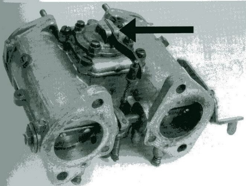
Dellorto accelerator pump mechanism.
