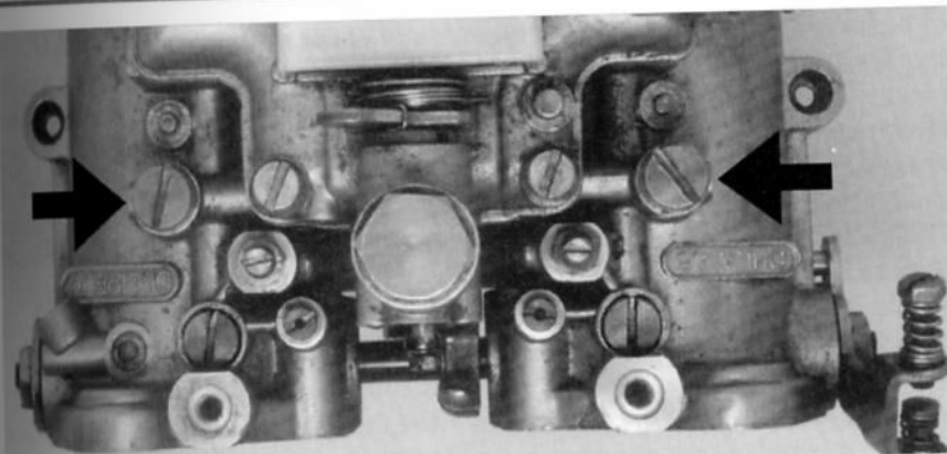
Dellorto accelerator pump cover plugs (arrowed).
