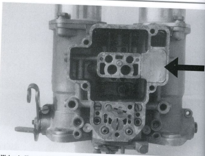
Weber baffle plate (arrowed) shown fitted. All is now ready for fitting of the top cover
