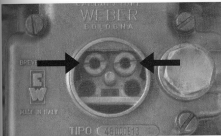
Weber emulsion tube holders (arrowed) fitted.
