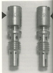
Dellorto idle jet holder. Note the positioning of the air bleed holes which control the idle mixture and the progression phase mixture strength. Size numbers arrowed.
