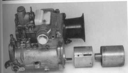
Choke and auxiliary venturi positioned in front of a Dellorto carburetor. Fit the choke first, then the auxiliary venturi.
