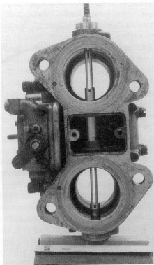
A spindle, with the bearing already pressed on, being tapped into the carburetor body. The other bearing has already been tapped into place. To prevent that bearing from moving, a washer is placed between the bearing and the flat surface of the vice top. This method requires assistance.
