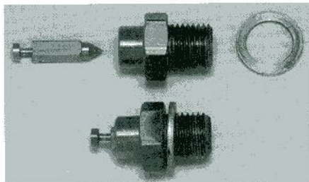
Needle and seat in assembled and component form.
