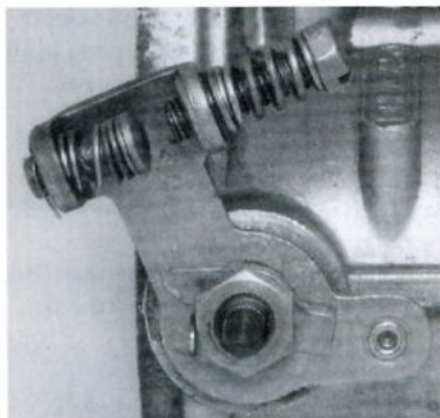
Dellorto throttle arm in position on the throttle spindle. Note raised tab to lock nut.
