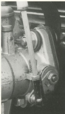
Far left - Throttle spindle in the idle position.
