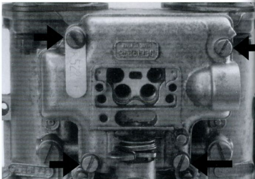
Carburetor top cover fitted and four securing screws (arrowed) tightened.
