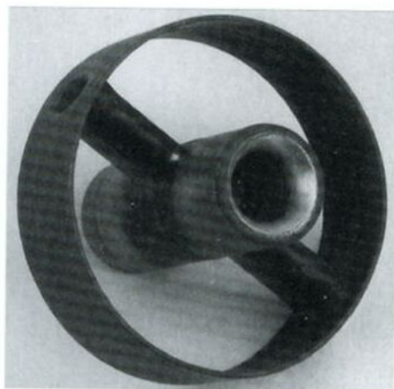
45 DCOE auxiliary venturi shown the right way around for installation in the carburetor. The small diameter of the nozzle must be front facing. Always check this.
