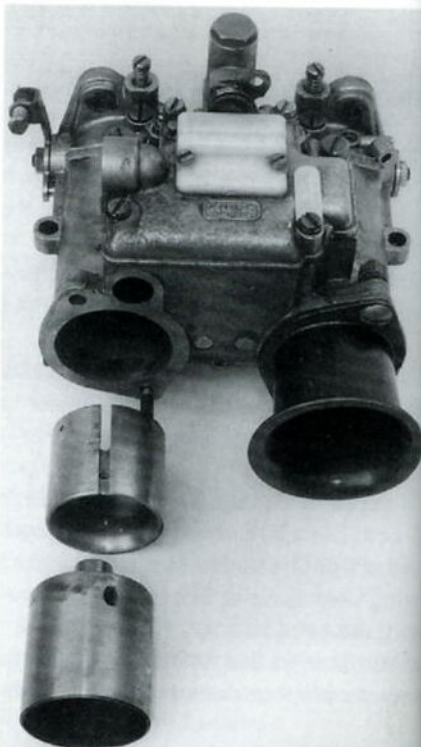
Dellorto DHLA carburetors with the choke and auxiliary venturi in front. Note the shape of the auxiliary venturi, the 40's (top) is slightly different to the 45/48's (above).
