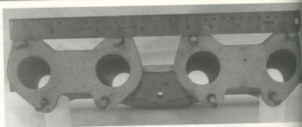
Use a straight edge to check that the studs are in alignment.
