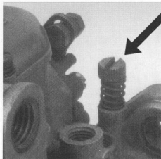
Exposed type idle mixture adjusting screw on a Weber. The Dellorto idle mixture adjusting screw is very similar.
