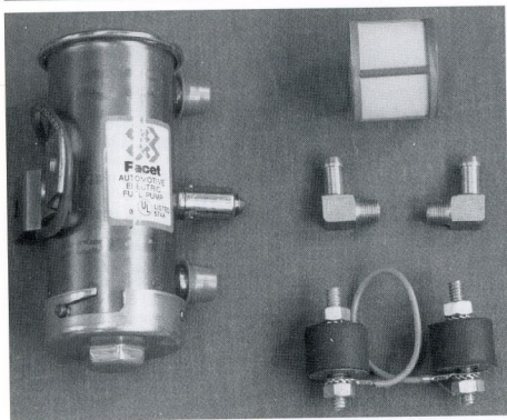
High-performance aftermarket fuel pump kit. (courtesy Peter Burgess).
