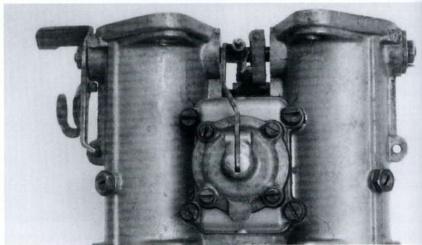
Dellorto accelerator pump bottom well cover fitted.
