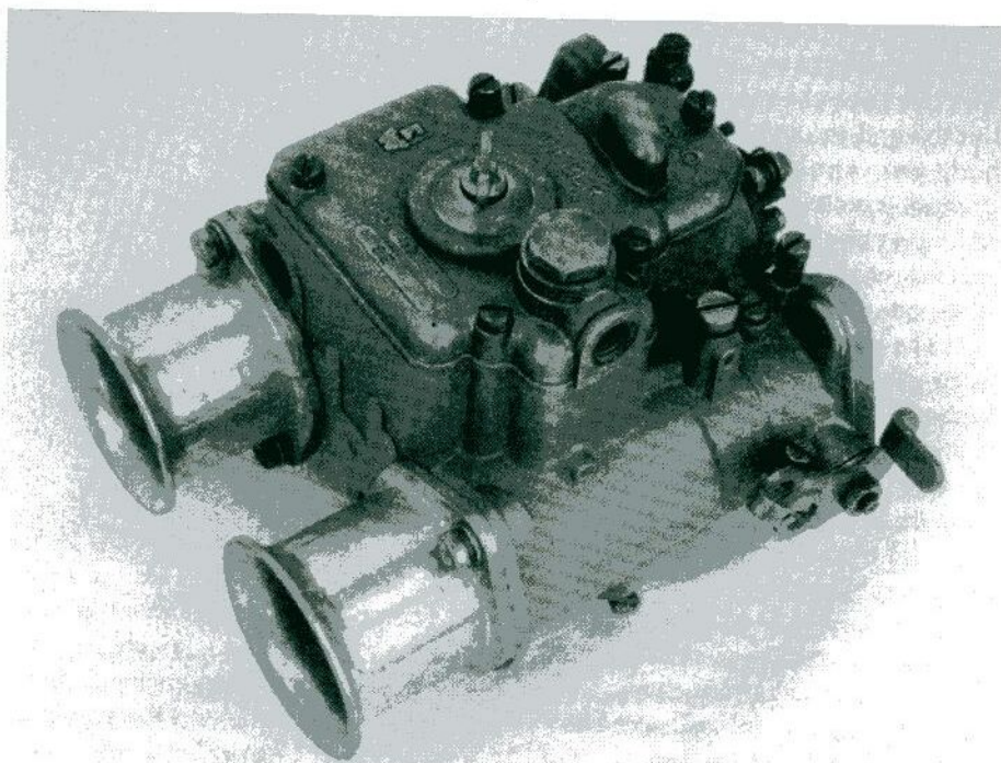
45 DCOE Weber.
