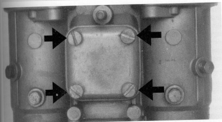
Weber bottom well cover fitted to the carburetor. Securing screws arrowed.
