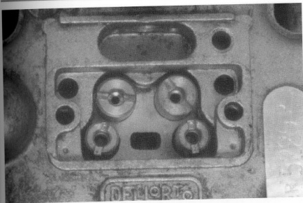
Dellorto carburetor top with the inspection cover off showing the emulsion tube holders and the idle jet holders.
