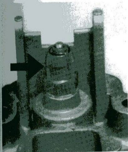
Weber needle valve and seat fitted into the top cover.
