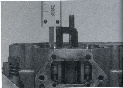
Below - Weber accelerator pump control rod height being measured.
