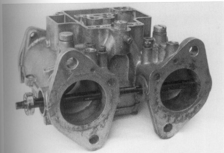
A new bearing in position on the spindle (which is there to act as a guide while the bearing is gently tapped into the carburetor body). The spindle just goes back as the bearing goes into the bore of the carburetor body.
