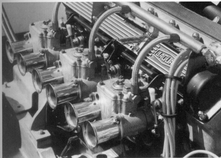
A trio of Webers on a racing Jaguar engine.
