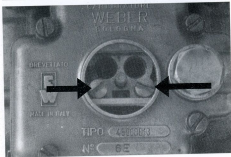
Below - Weber carburetor with cover removed showing the position of the idle jets.
