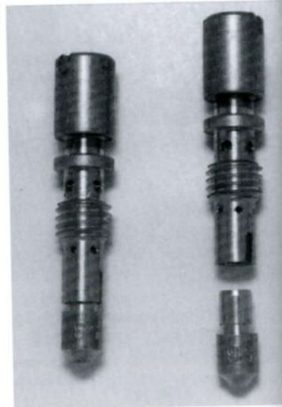
Weber (top photo) idle jet and holder assembled (left) and separated (right).
