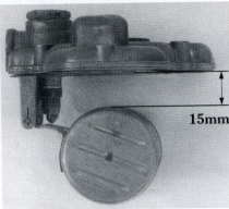
Weber floats being set to 15mm droop.
