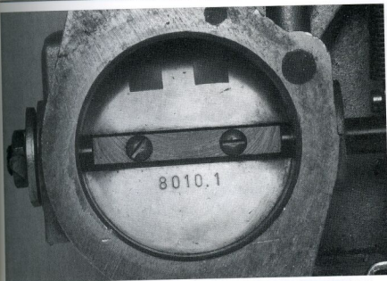
Dellorto butterflies with the progression hole sweep slots and the numbers clearly visible.
