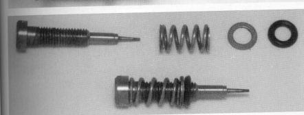
Dellorto idle mixture screw components (above) and correctly assembled (below).
