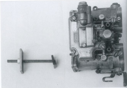
Photos show a simple-to-make puller for the removal of jammed chokes.
