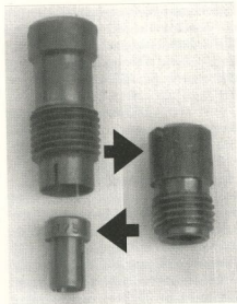
Weber air corrector (left) and Dellorto holder (right). Position of the sizing numbers arrowed.
