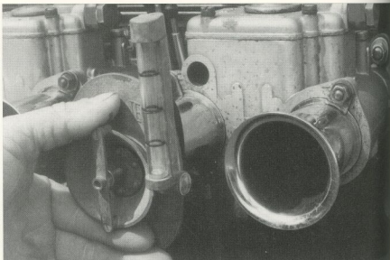
"Motometer" being used. This type of flow meter fits over the end of the trumpet. The sight reading glass is integral with the meter.
