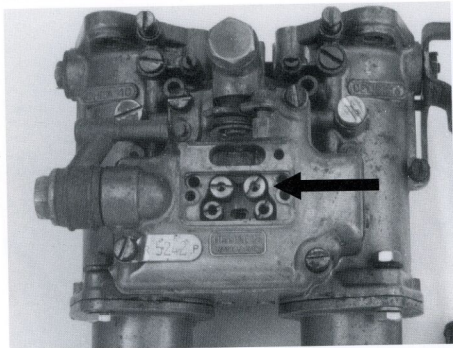
Top of a Dellorto with the jet inspection cover removed and showing the emulsion tube holder which in turn holds the actual emulsion tube, main jet and air corrector.
