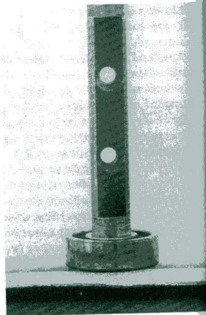
Photos show a spindle being tapped into a new bearing. Use a copper hammer or an aluminum drift to tap the spindle into the bearing. The spindle is guided to a large degree, but do make sure the spindle is square to the bearing and that the bearing is placed flat on the top of the vice jaws.
