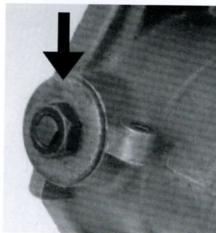
Right - Weber plain cover (arrowed) and nut fitted to the end of the throttle spindle.
