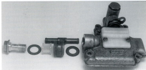
Below - Components of the integral Dellorto fuel filter.
