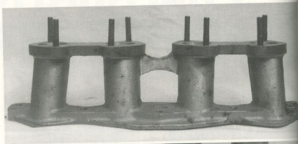
Use a straight edge to check that the studs are in alignment.
