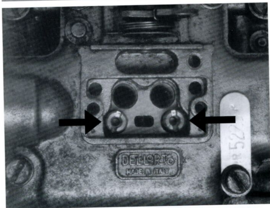
Dellorto carburetor with cover removed and showing the position of the idle jets.
