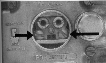
Weber idle jet holders (arrowed) fitted.
