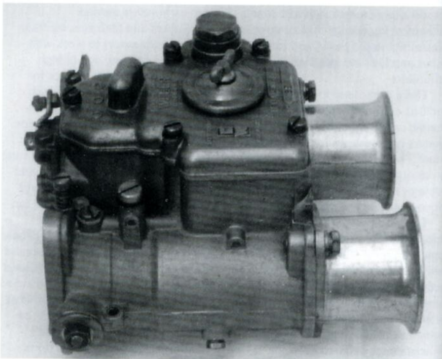
45 DCOE Weber.
