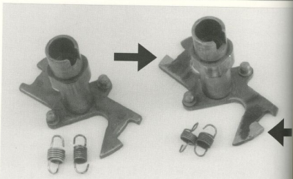
If the engine is set up with 15 or 16 degrees of advance at idle, the total advance will have to be limited. This is achieved by braising the advance slot (arrowed right) which reduces the amount of travel. In this case the slot is reduced by 2mm so that the total advance does not exceed 35 or 36 degrees. Note the light springs which allow total advance at about 3300rpm.
