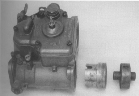
Weber 40 DCOE carburetors with the chokes and the auxiliary venturis shown in front. The shape of the 40's (top) auxiliary venturi is different to the 45/48's (above).
