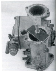
A choke puller installed. The puller's bottom plate is behind the choke to be removed and the nut is about to be tensioned. The carburetor body may have to be heated to get the choke to move.
