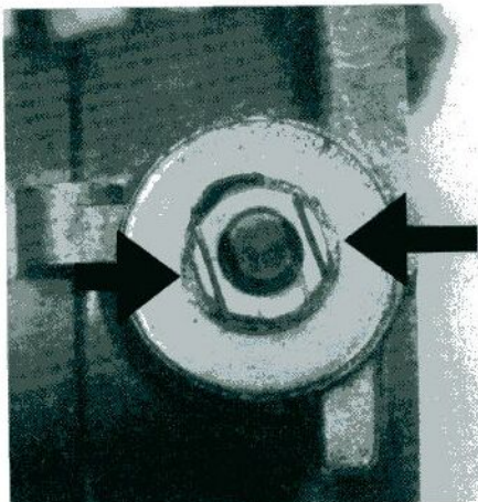
This nut has been cut in two places to release it from the spindle. Always cut off tight nuts to prevent spindle damage: nuts are cheap, spindles are not!
