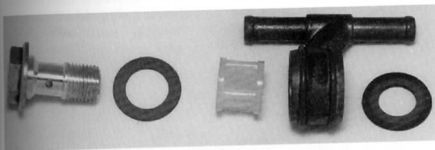
Dellorto integral fuel filter and fuel union components.
