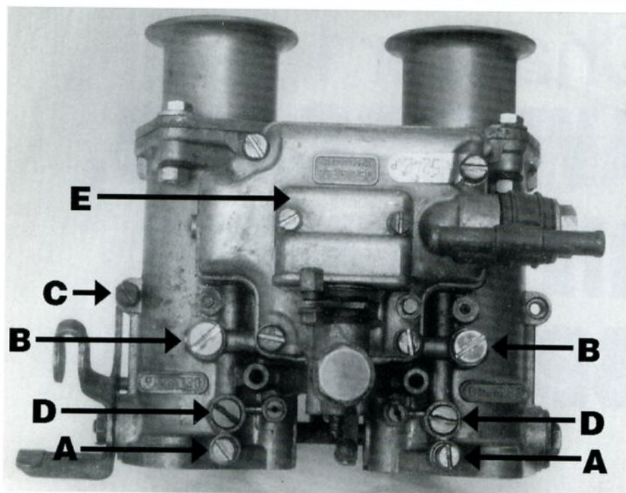
View of a Dellorto showing the idle mixture adjusting screw at (A) the pump jet screw cover at (B) the throttle arm adjustment screw at (C) the progression hole screw cover at (D) the main jet and jet cover at (E).
