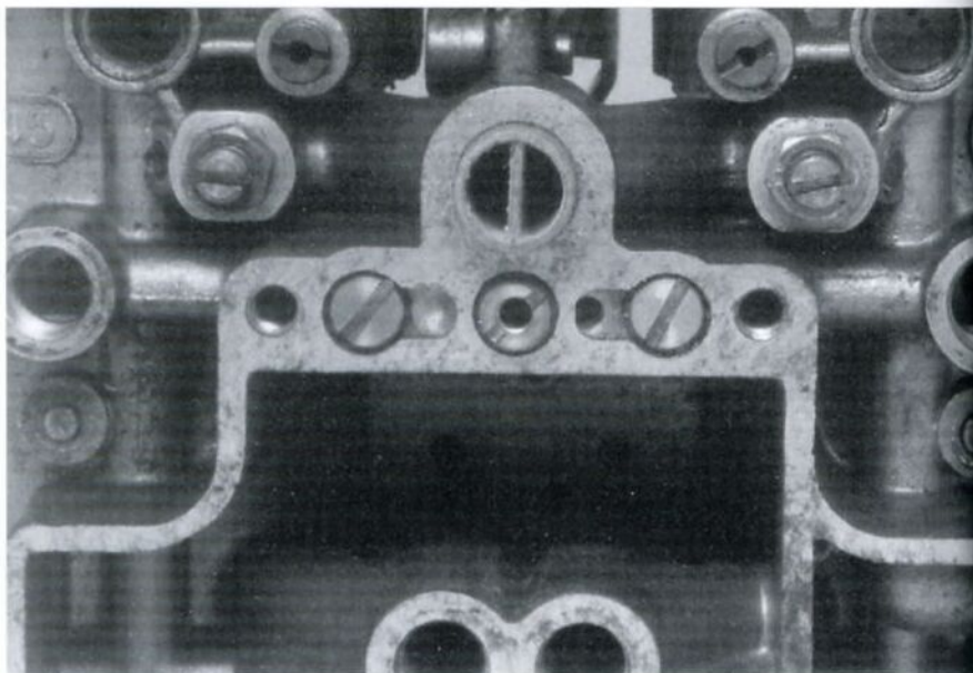
The jetting that has to be in place before the top cover is fitted.
