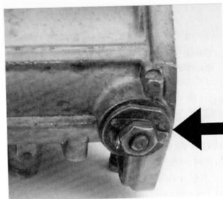
Dellorto with plain throttle spindle cover (arrowed) correctly fitted. Note how tab of lockwasher is turned up to lock nut.
