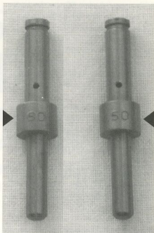
Weber accelerator pump jets. Position of size numbers arrowed.
