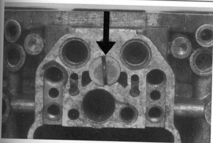
Weber spindle return spring anchor plate (arrowed) correctly fitted.
