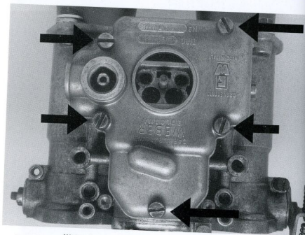
Weber top cover fitted. Arrows show securing screws.
