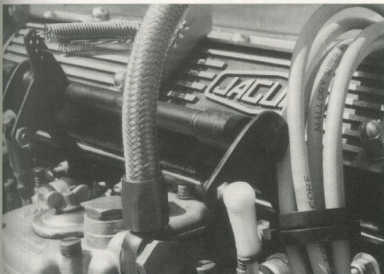
Main throttle bar at full throttle position. Note the downward angle of the main bar's throttle arms. Ideally, the arm's arc of travel is set so that the arc's center coincides with the horizontal plane.
