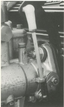
A typical double-socket pushrod as commonly used on throttle bar systems. It is essential that the socket-to-socket dimensions of all pushrods are identical.
