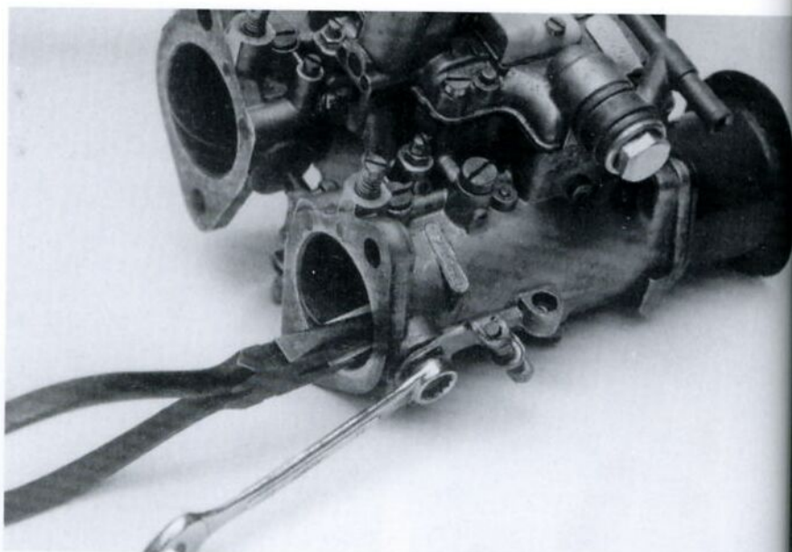
A pair of long-nosed pliers holding butterfly/spindle (with alloy shim between the pliers' jaws) while the spindle nut is tightened.
