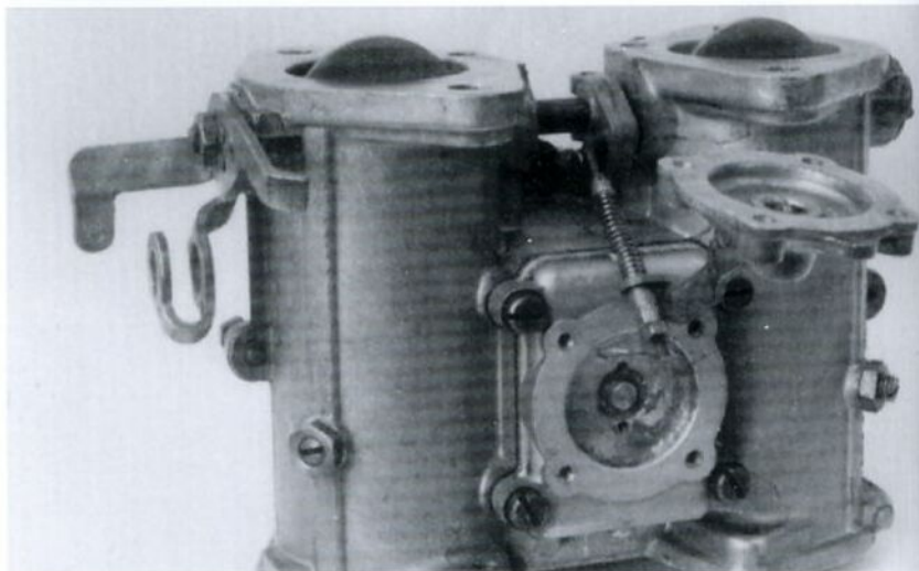
Dellorto accelerator pump bottom well cover fitted to actuating rod.
