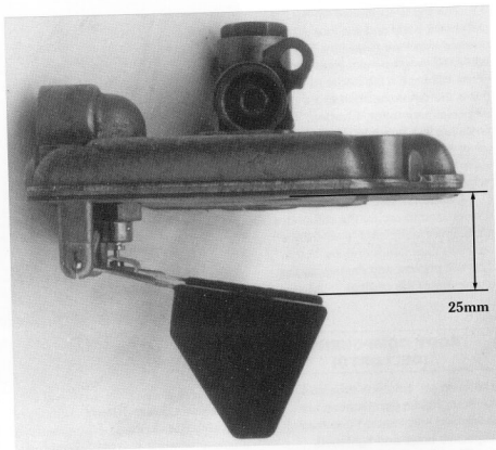
Dellorto floats being set to 25mm droop.
