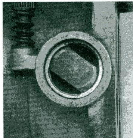
Outer bearing race ground away enough to allow a specially made piece of flat bar to neatly fit into the bearing and be turned 90 degrees. A long drift can be used to push against the flat bar with the knowledge that it is securely locked into the race. Heat the carburetor body before shifting the race.
