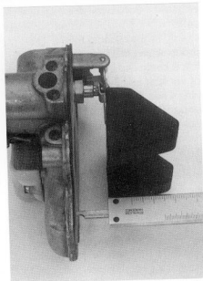
Dellorto floats being set at 15mm when the needle is just seating.
