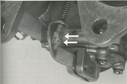
Dellorto accelerator pump actuating rod and arm showing the two nuts (arrowed) that are used to adjust the position of the arm which contacts the accelerator pump diaphragm.
