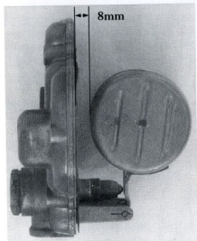
Weber floats being set to 8mm with the needle and seat just touching.
