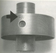
Weber auxiliary venturi. Position of sizing numbers arrowed.
